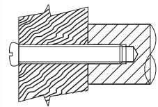
bolt-through fixing
