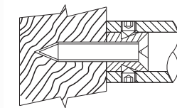
concealed fixing
