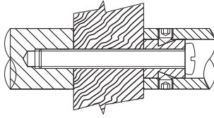
back to back fixing
