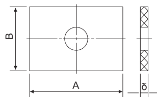
Square washer
