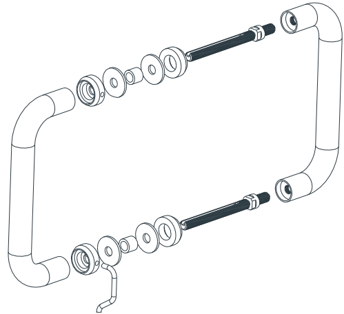
Back to back fixing, thread type
