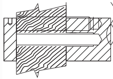
bolt-through fixing fixing nuts with cover caps
