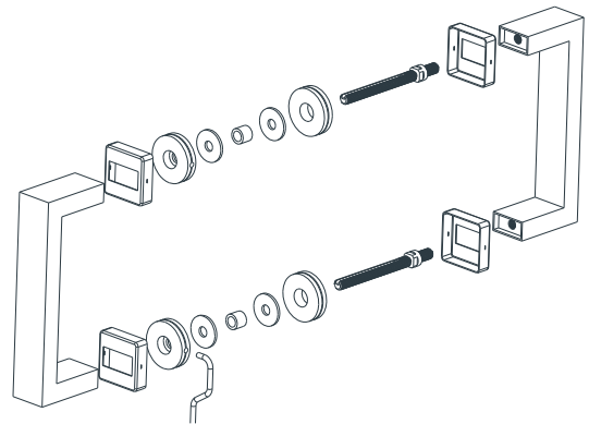
Back to back fixing, thread type
